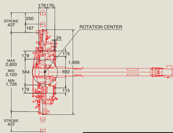
Drawing: UR-W234 (Unit: mm)
